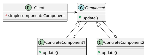
Figure 312: Diagram of the Component Design Pattern
